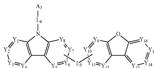
[Chemical Formula 3]
