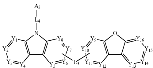
[Chemical Formula 3]
