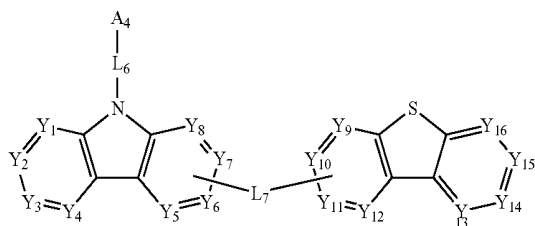
[Chemical Formula 3]
