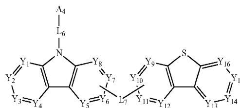
[Chemical Formula 4]
