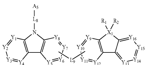
[Chemical Formula 5]
