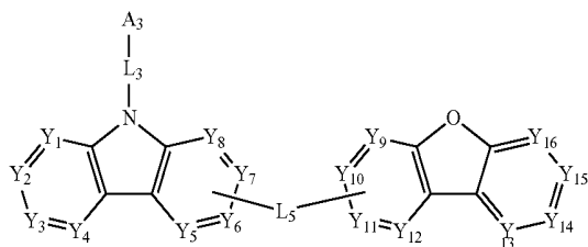
[Chemical Formula 3]
