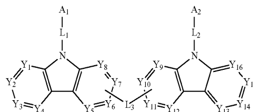
[Chemical Formula 2]
